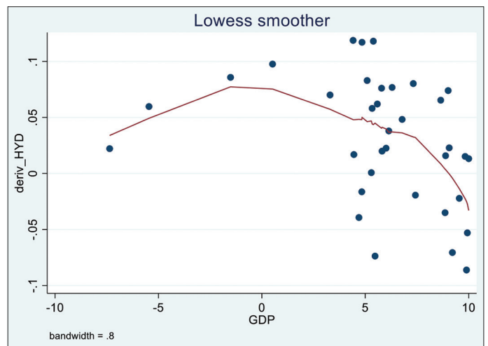
Figure 4: Description of pointwise marginal effect for hydroelectric generation
