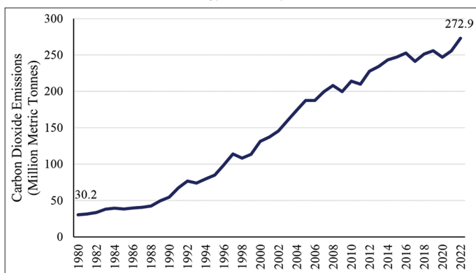
Figure 1: Carbon dioxide (CO 2 ) emissions from the use of fossil fuel energy in Malaysia
