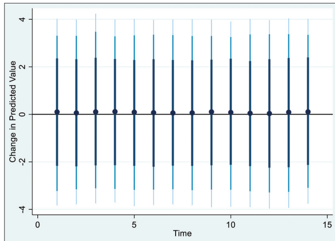
Figure 2: Expected shock results in hydroelectric generation using dynamic ARDL simulation. Model of the change ( \pm 1\% ) in the forecast of hydroelectric generation on economic growth (GDP). The dot indicates the average forecast value, and the gradient from dark blue to light blue represents the 75, 90, and 95% confidence intervals.
