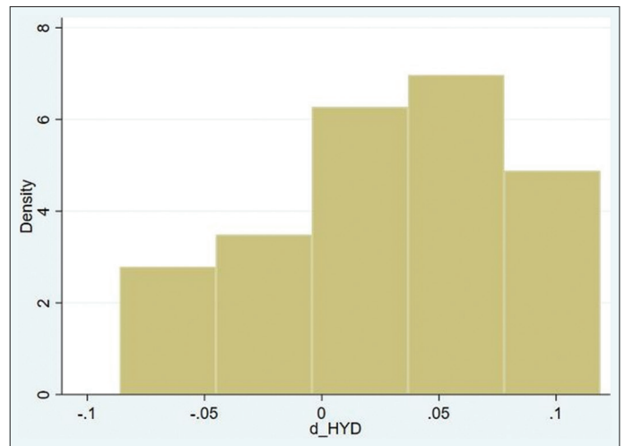
Figure 3: Distribution of pointwise marginal effect
